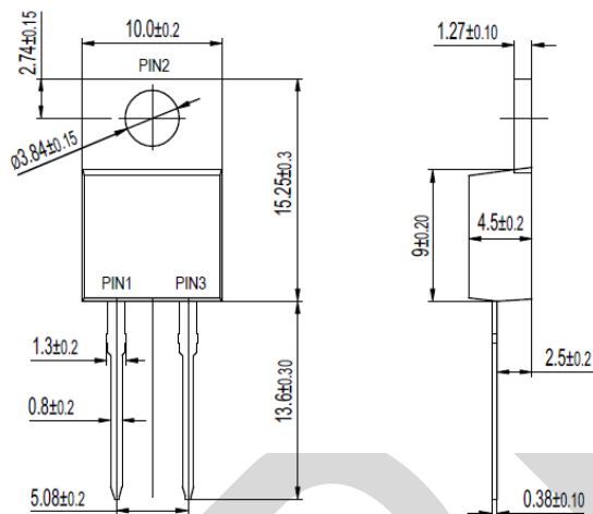
TO-220ACT Dimensions in millimeters
