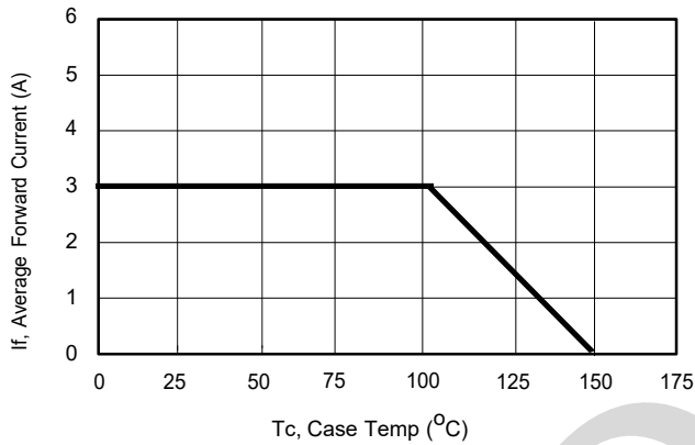
FIG.1: Current Derating, Case
