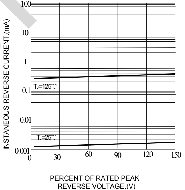
FIG.4-TYPICAL REVERSE CHARACTERISTICS
